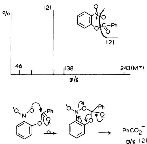
FIGURE 5. Negative ion mass spectrum of o -nitrophenyl benzoate. Experimental conditions: 70 eV, source pressure 2 \times 10^{-6} torr, accelerating potential -3.6 kV.
