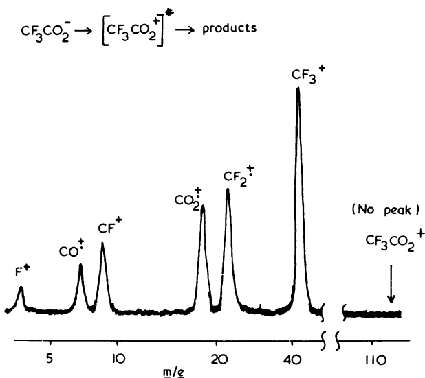
FIGURE 3. Dissociative charge inversion spectrum derived from the CF_3CO_2^- ion of (CF_3CO)_2O . Hitachi Perkin Elmer R.M.U. 6D mass spectrometer, electron energy 70 eV, accelerating voltage -3.6 kV, sample pressure 2 \times 10^{-6} torr in the source, and collision gas ( N_2 ) pressure of 1 \times 10^{-5} torr in the second field-free region. Decompositions occurring in the second field-free region. Electric sector set to transmit main beam of negative ions, magnet transmits positive ions, spectrum produced by magnetic field scan.
