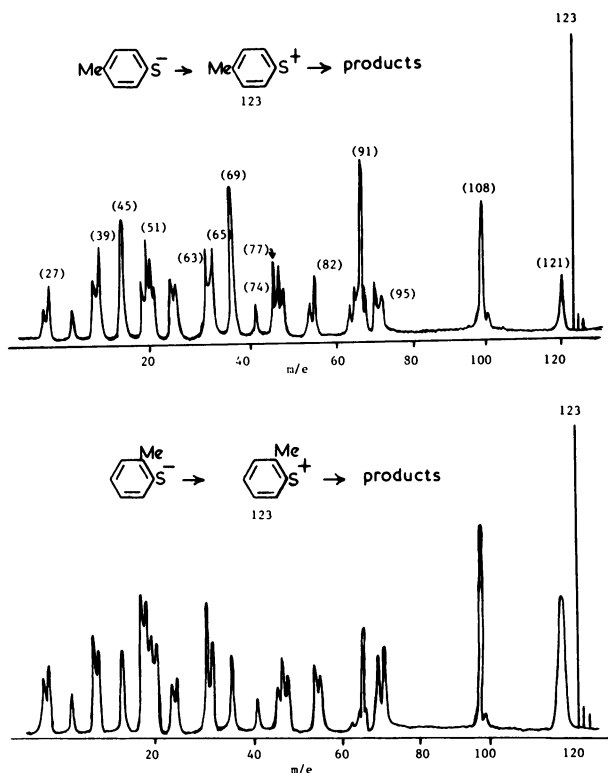
FIGURE 4. Dissociate charge inversion spectra of (a) p - \text{MeC}_6\text{H}_4\text{S}^- from (p\text{-MeC}_6\text{H}_4\text{S})_2 and (b) o - \text{MeC}_6\text{H}_4\text{S}^- from (o\text{-MeC}_6\text{H}_4\text{S})_2 . Experimental conditions as recorded in the legend to Figure 3. Peaks are shown with the conventional masses in brackets.
